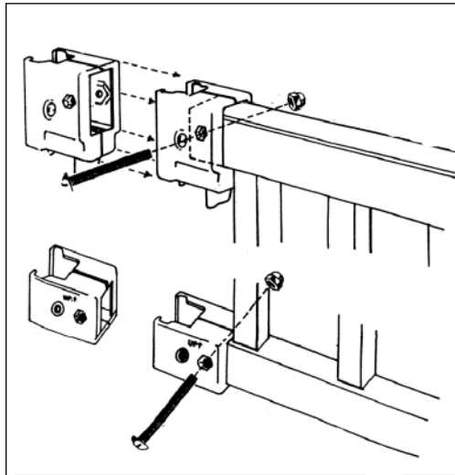
PH53 Upper Track
